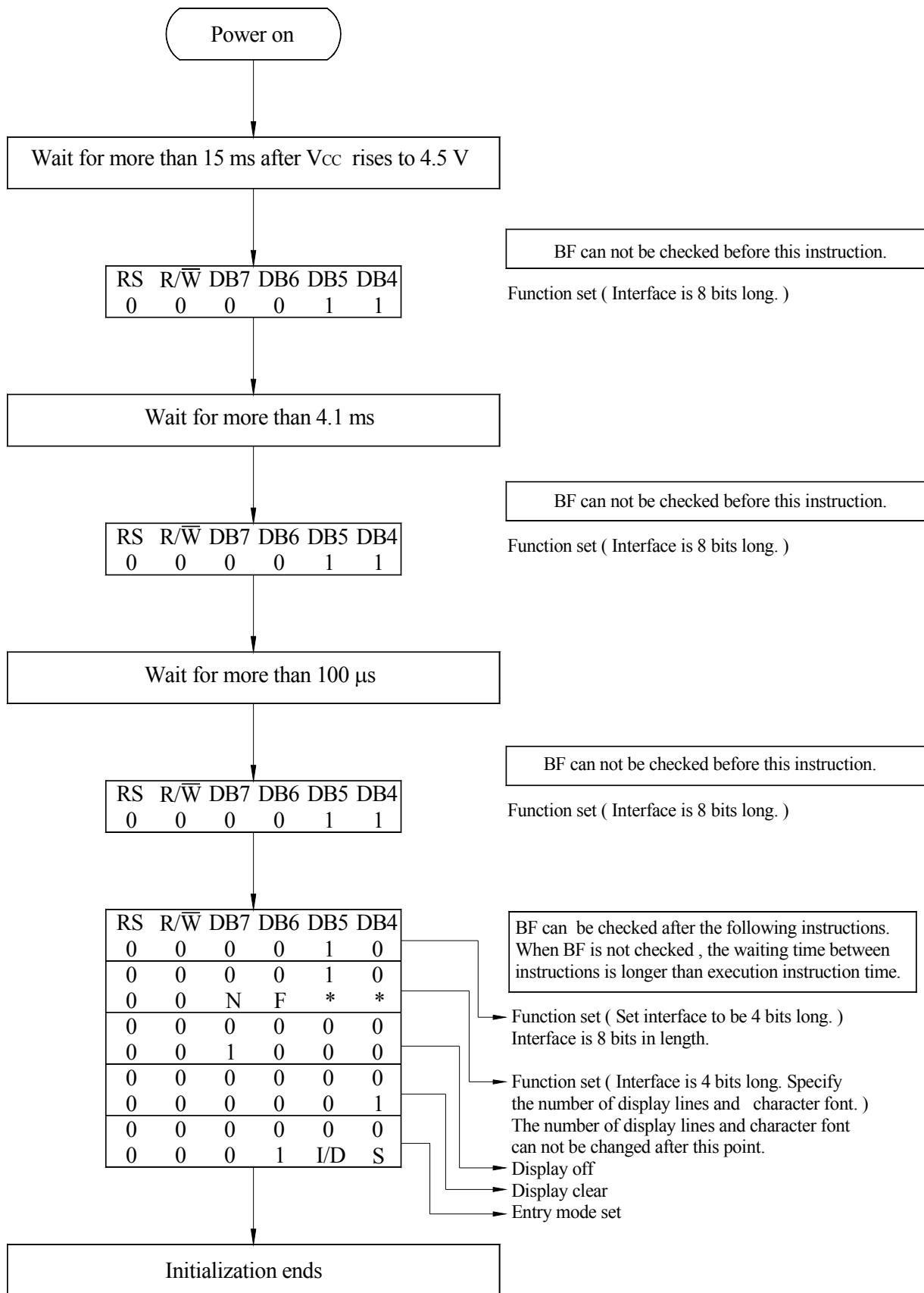
4-Bit Ineterface
