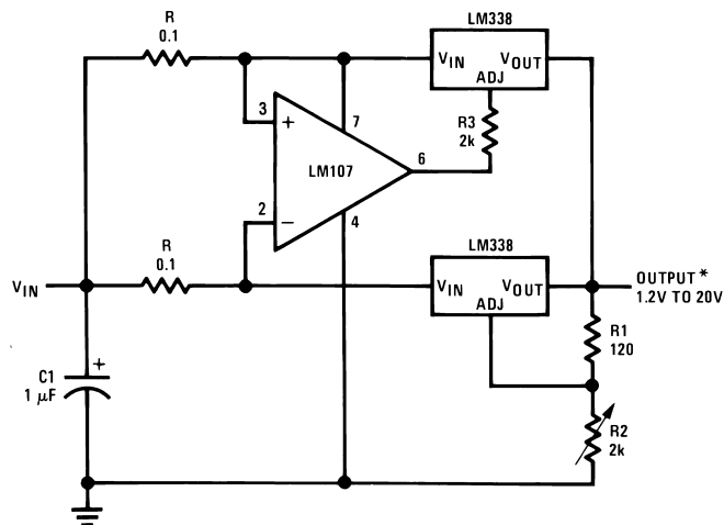
10A Regulator
