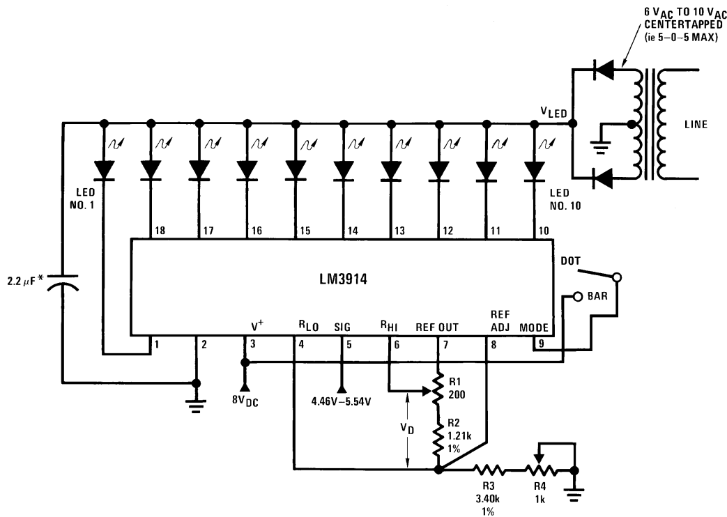
Expanded Scale Meter, Dot or Bar
