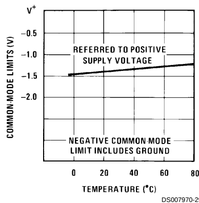
Common-Mode Limits
