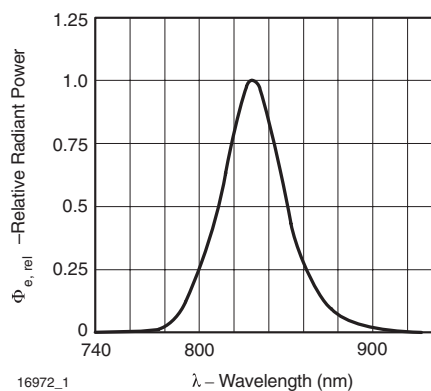
Figure 7. Relative Radiant Power vs. Wavelength
