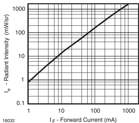
Figure 5. Radiant Intensity vs. Forward Current
